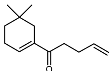
4-Penten-1-one, 1-(5,5-dimethyl-1-cyclohexen-1-yl)-
